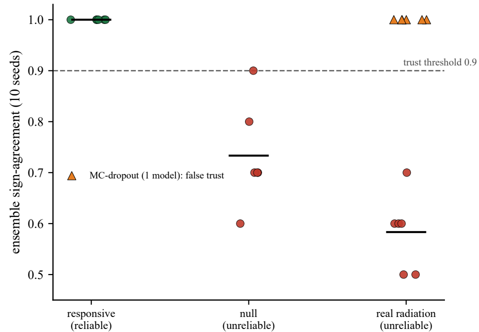
(a) cheap ensemble indicator separates reliable / unreliable
