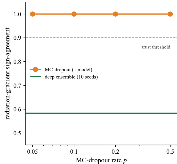
(c) dropout is over-confident at every rate
