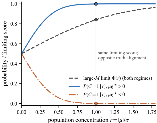
(b) Mean-aligned agreement is scale-free but bias-blind
