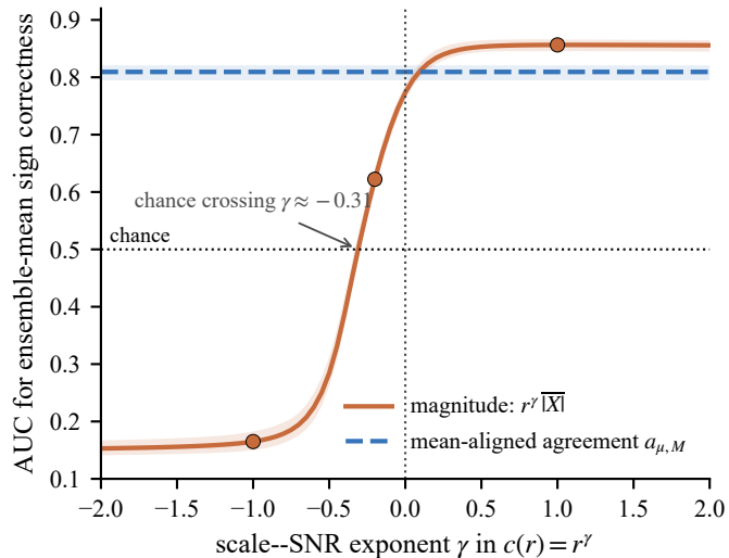
(a) Magnitude inversion has a data-dependent crossing
