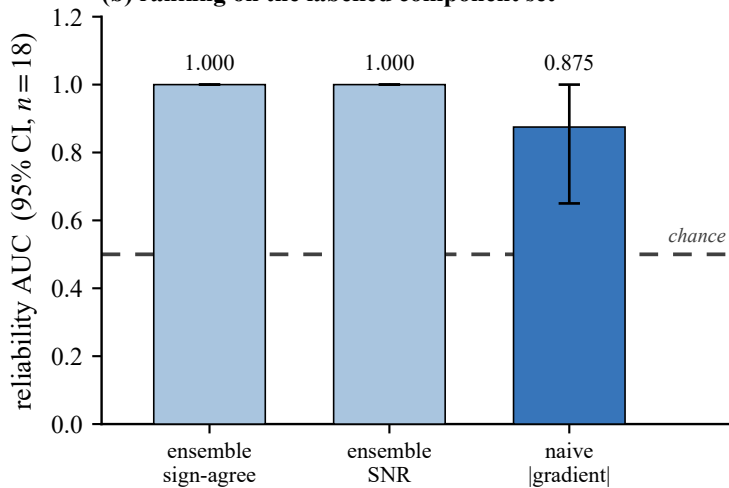
(b) ranking on the labelled component set
