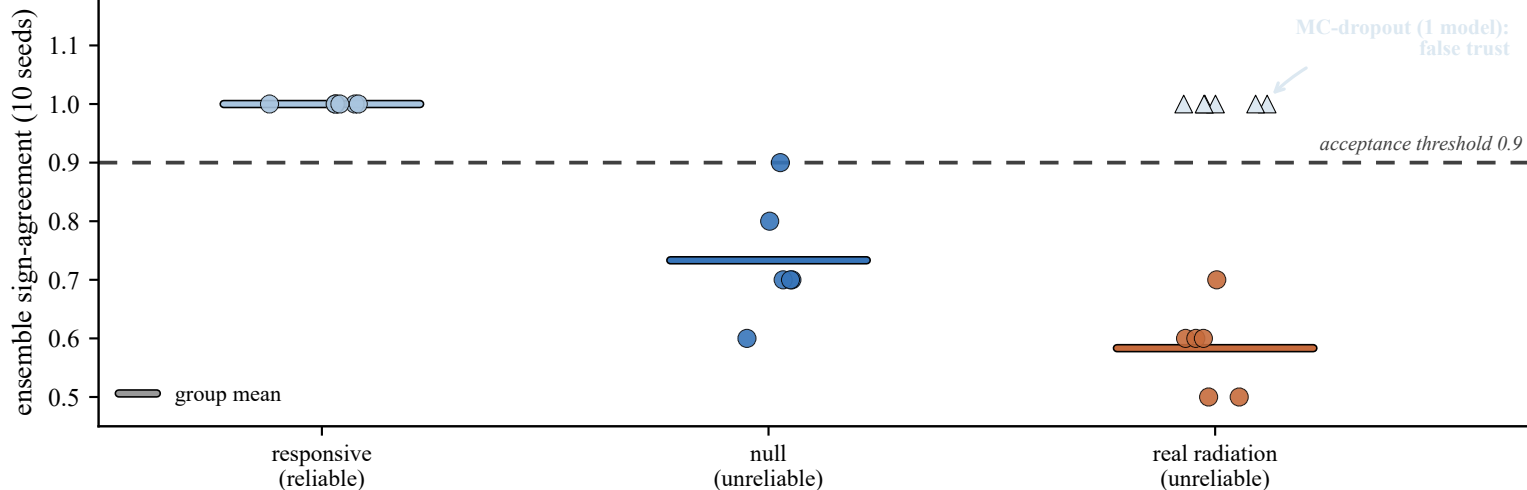
(a) cheap ensemble indicator separates reliable / unreliable
