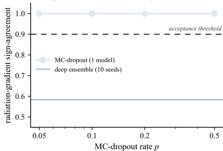
(c) dropout is over-confident at every rate
