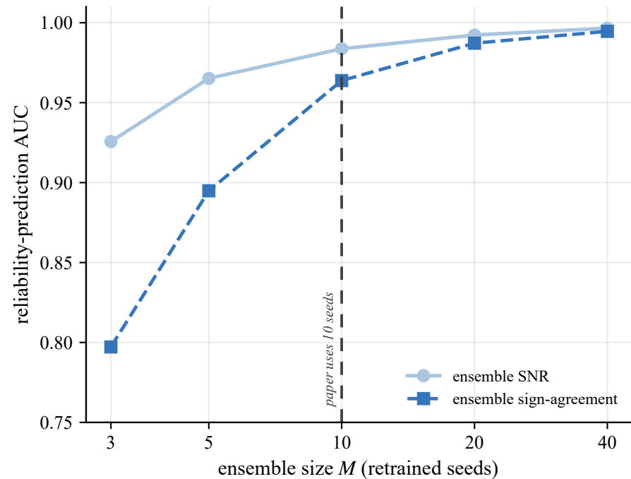
(a) controlled-model discrimination versus ensemble size
