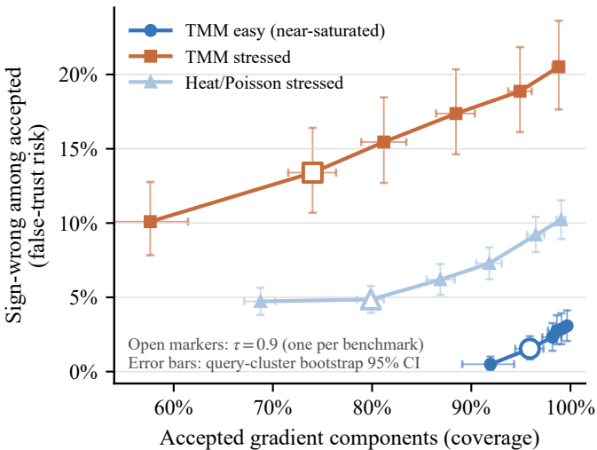
(a) Selective risk versus accepted coverage
