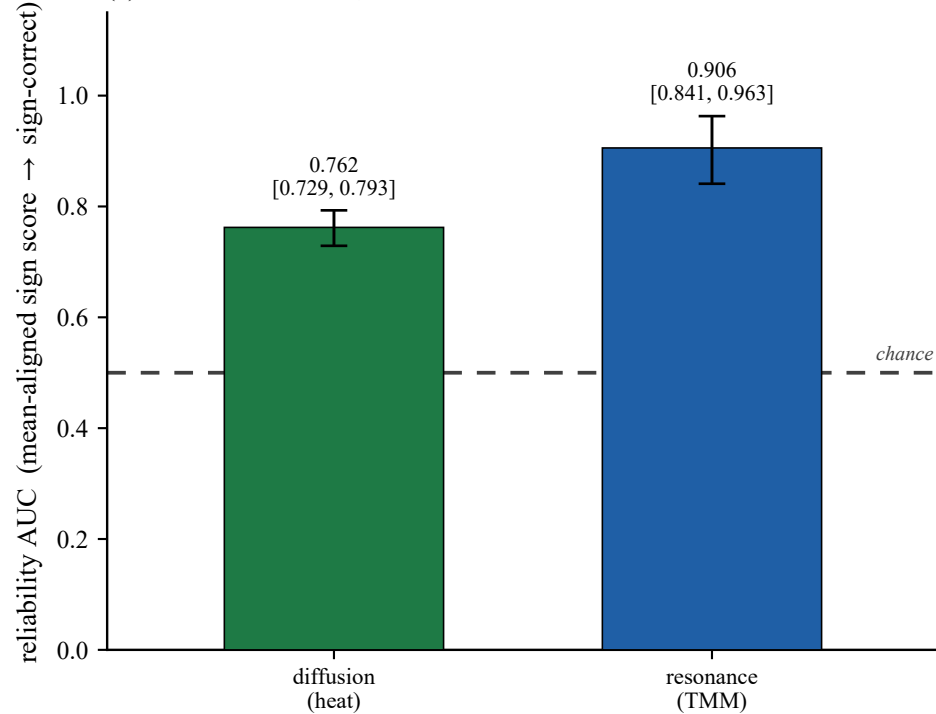
(b) above chance in both, but diffusion is weaker
