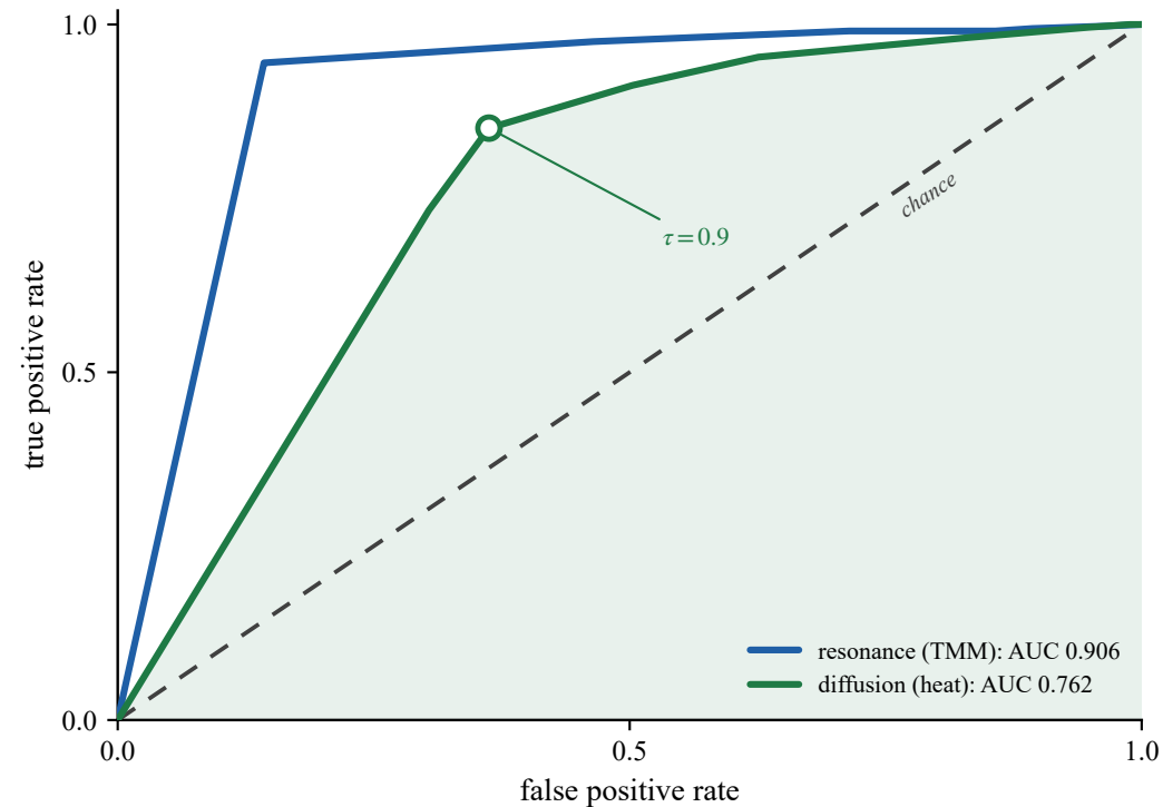
(a) the ranking generalises to diffusion, weaker than resonance
