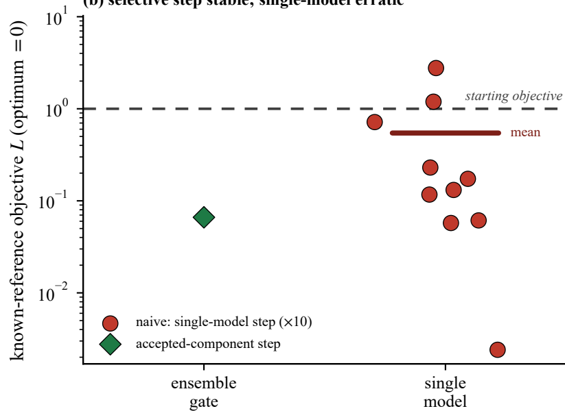
(b) selective step stable; single-model erratic
