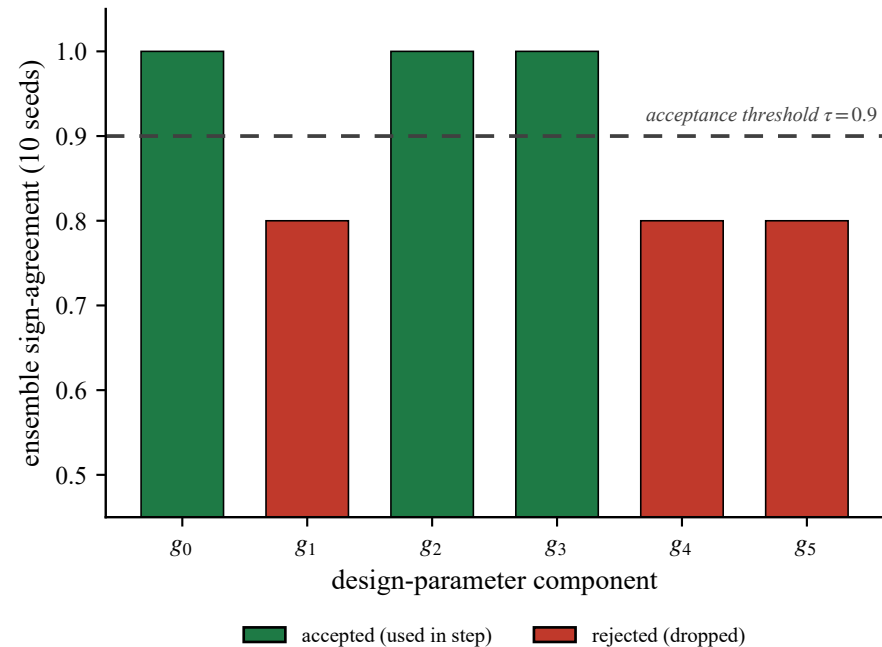
(a) score rejects seed-unstable components
