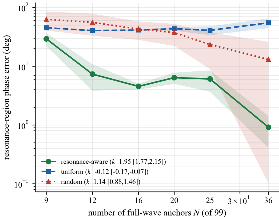
Advantage recurs on a second cell topology (cross dipole)
