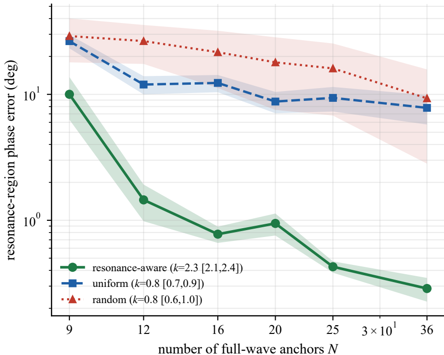
Data efficiency (20 seeds, mean \pm std)
