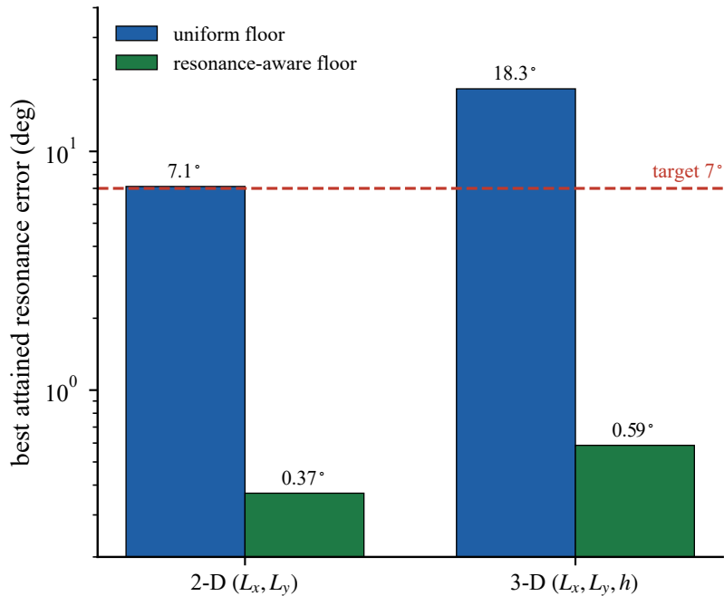
(b) curse-of-dimensionality bite
