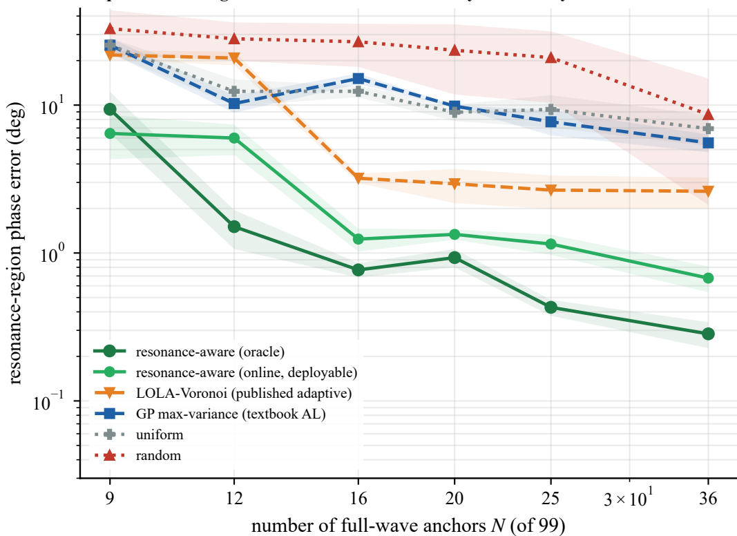
Acquisition strategies: the resonance-aware family beats every off-the-shelf rule
