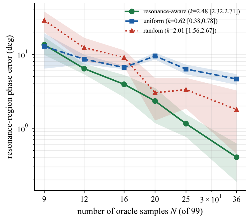
(a) driven oscillator / series-RLC (non-EM)
