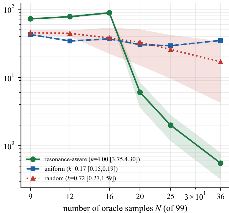
(b) Fano resonance line shape (non-EM)
