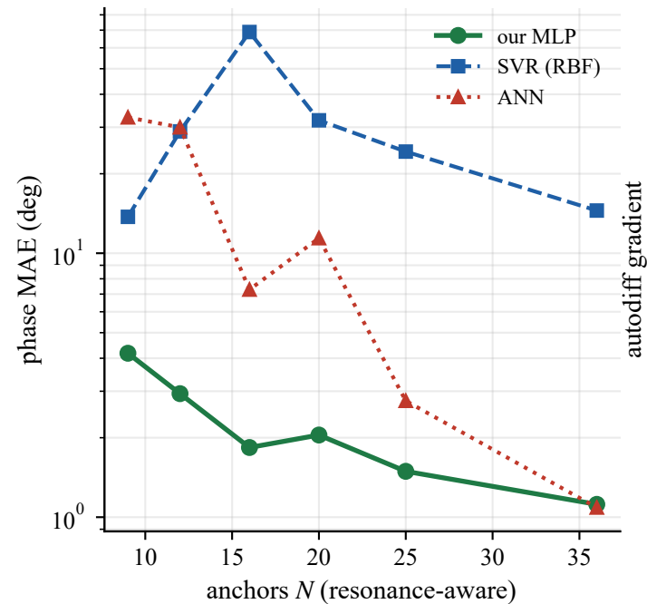
(a) surrogate vs ML baselines
