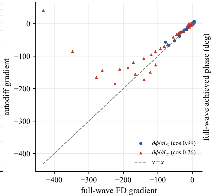
(b) differentiable gradient validation
