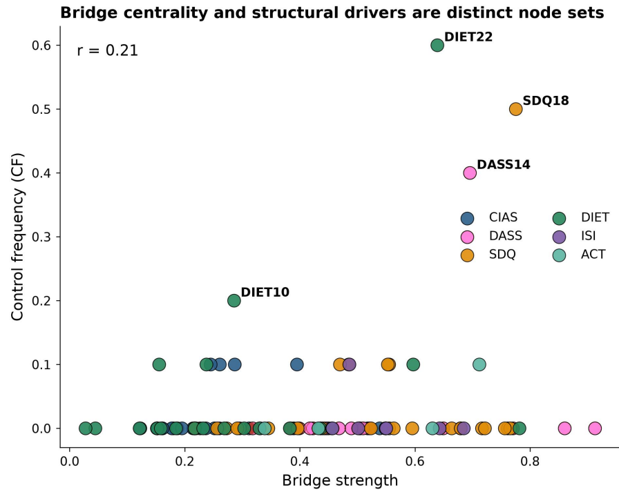
Supplementary Figure S4. Bridge strength versus control frequency: bridge-centrality nodes and structural-control nodes are distinct ( r = 0.21 ). CF, control frequency.
