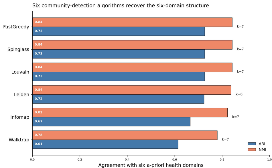
Supplementary Figure S18. Community partitions were broadly aligned with the six prespecified domains. Leiden returned six communities, whereas the other five algorithms returned seven. ARI and NMI between each algorithm’s data-driven partition and the six a-priori domains; k is the number of communities returned. Leiden returns exactly six communities.
