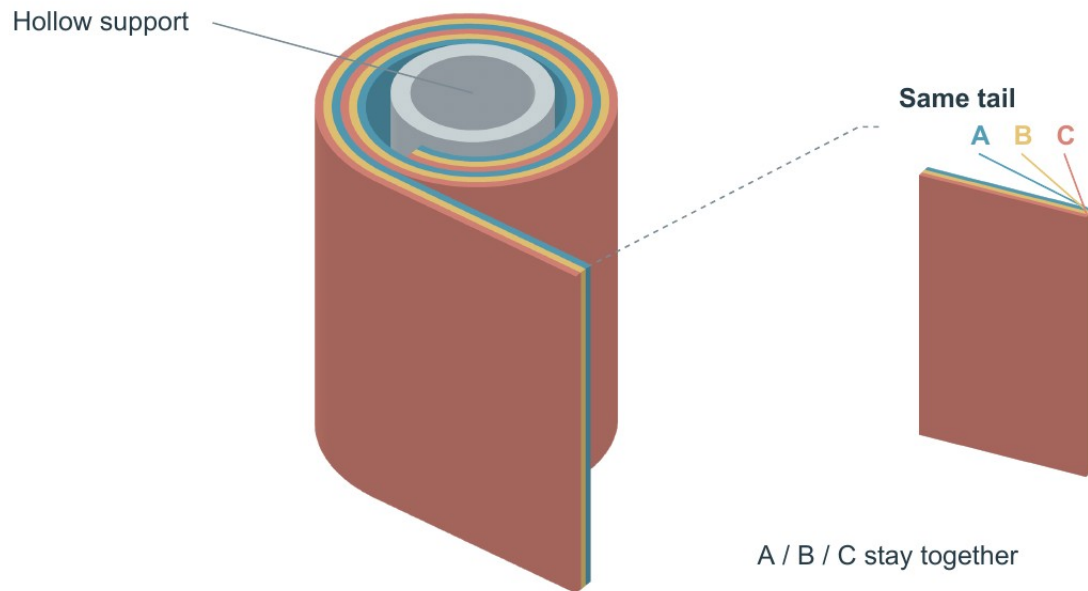
Figure 1. Co-wound laminate DEMO. Blue, gold, and coral identify layers A, B, and C. The enlarged view repeats the same straight tail; the hollow core is a separate neutral body. Dimensions are illustrative, without physical units.
