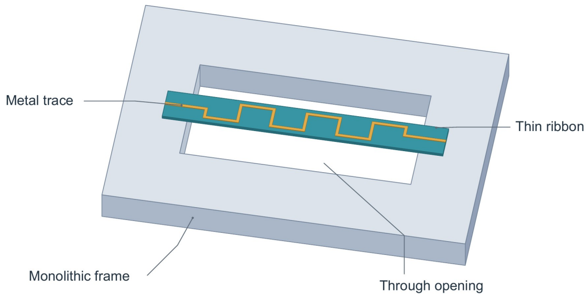
Figure 1. Suspended-ribbon geometry DEMO. An orthographic view shows a monolithic frame with a rectangular through-opening, a continuous ribbon contacting the frame at both ends, and a continuous metal trace on the ribbon's upper surface. The opening has no bottom plate, and the central ribbon span has no supporting pillar. Colors identify the three entities; fine gray leaders identify features without implying physical transport. The geometry is fictional and carries no measurement units or performance data.
