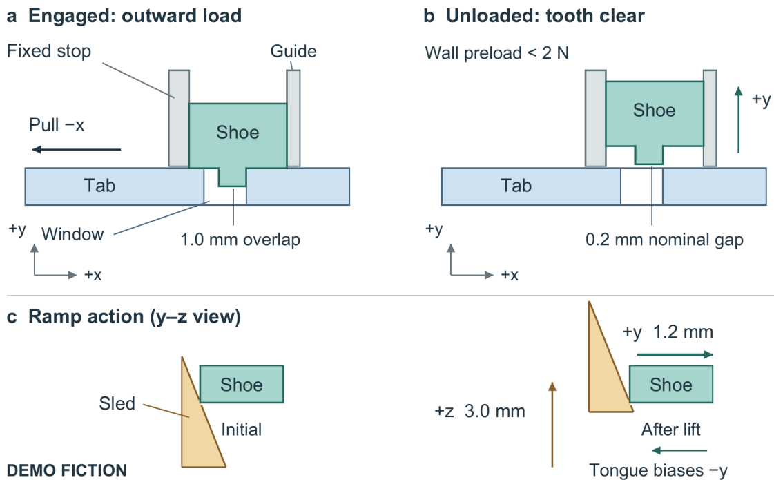
Figure 1. Stop-supported retention and transverse release in D — DEMO FICTION. The two upper views show the same tab, shoe, and fixed stop in the x - y plane; +z is out of the page. The lower paired y - z views show the same ramp and shoe before and after the lift, at the same scale and shoe height; they are not additional parts. Arrows distinguish outward loading from sled and shoe motion. Geometry is schematic, not a manufacturing drawing; the complete housing, integral return tongue, and underside relief slot are omitted. Release requires wall preload below 2 N. The figure depicts specified contact and motion, not a measured force partition.
