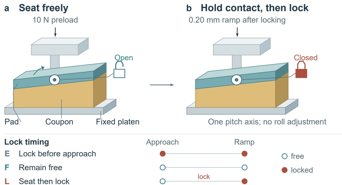
Figure 1. Use the same pitch freedom to seat the pad, then lock it for loading. The two views show mode L: seat at 10 N, hold and acknowledge preload, close the clamp without lifting, then zero and ramp 0.20 mm. Lock symbols denote clamp state, not internal construction. The strip compares E, F and L; open and filled circles mean free and locked. The pin permits only pitch. Perspective and slope are schematic, not measured geometry or pressure maps.
