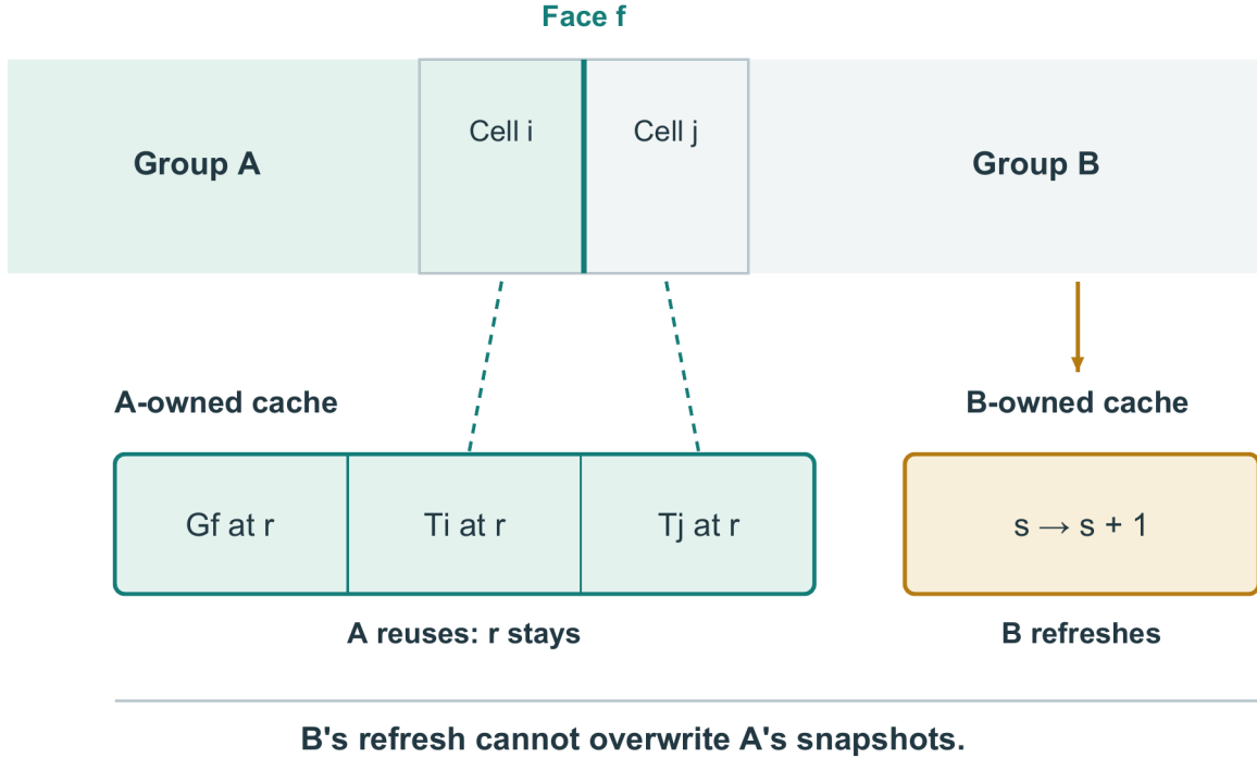
Figure 1. A boundary face retains its owner's refresh history. The cells are a detail of different 16 \times 16 groups; i < j assigns face f to A. Dashed lines link endpoints to their stored temperatures at A's refresh r . If A reuses while B refreshes at its own counter s , A's coefficient and both snapshots stay at r . The counters r and s are independent.
