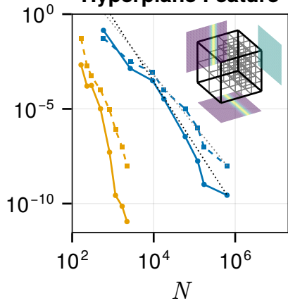
Hyperplane Feature
