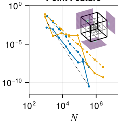
Point Feature
