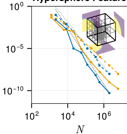
Hypersphere Feature
