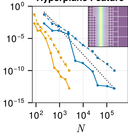
Hyperplane Feature
