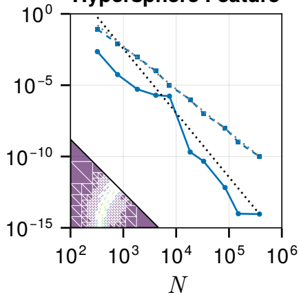
Hypersphere Feature
