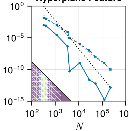
Hyperplane Feature
