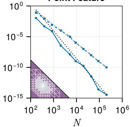
Point Feature
