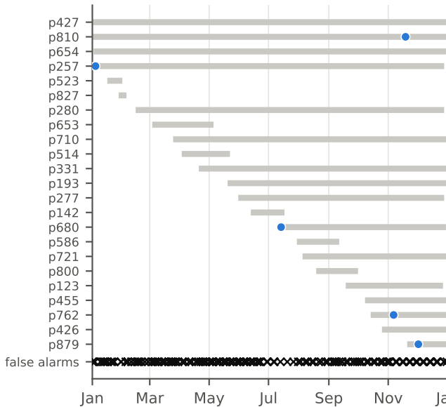
GNN: 5 of 23 found, 160 false alarms
