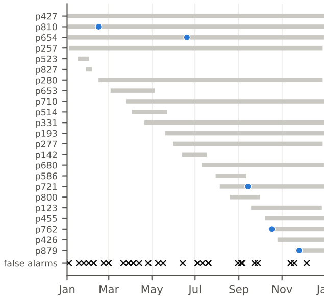
GNN: 5 of 23 found, 26 false alarms
