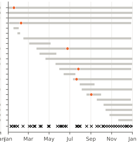
Ridge: 6 of 23 found, 47 false alarms
