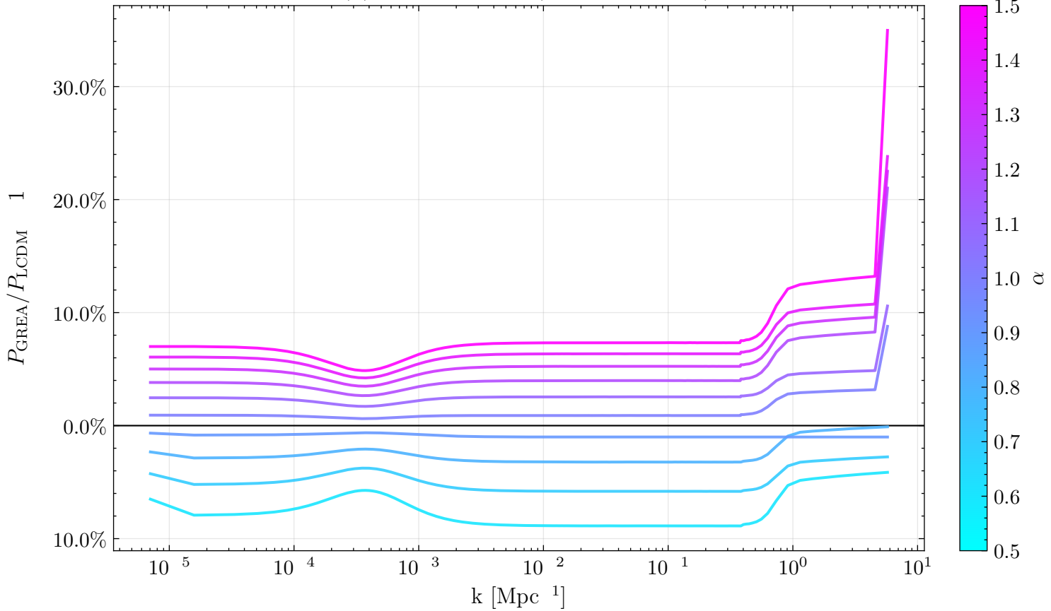
P(k) ratio at z = 0 (alpha variation)
