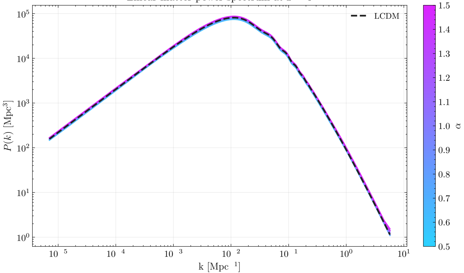
Linear matter power spectrum at z = 0
