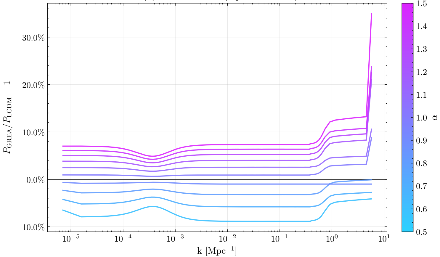
P(k) ratio at z = 0 (alpha variation)
