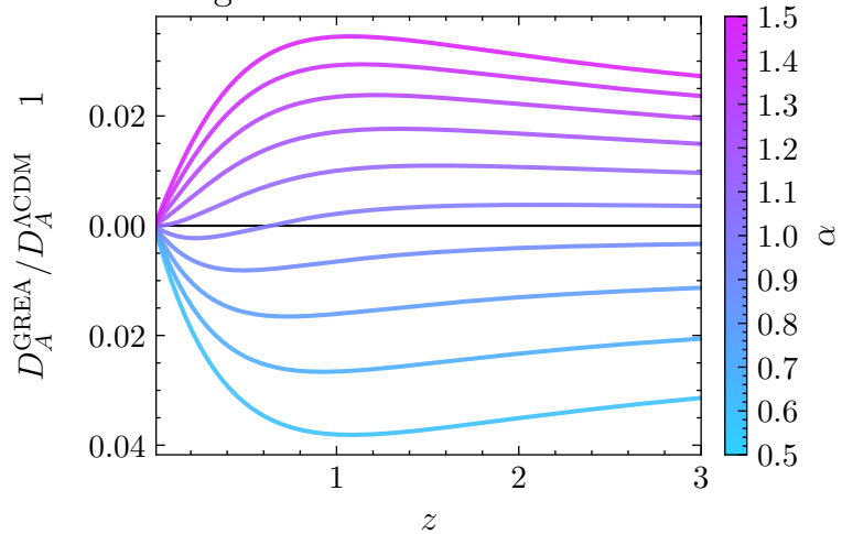
Angular diameter distance ratio
