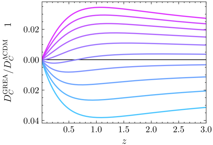
Comoving distance ratio
