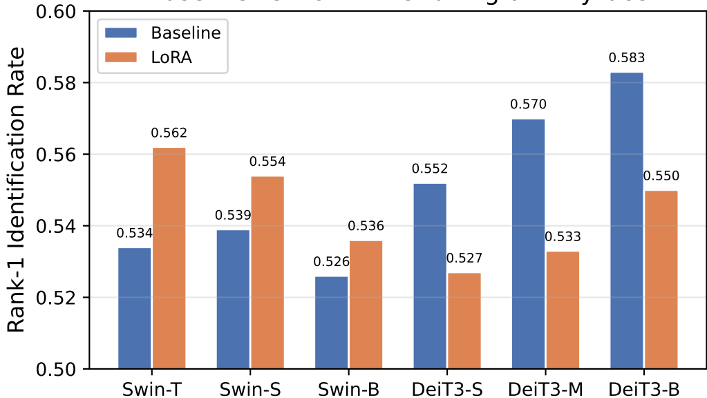
Baseline vs. LoRA Fine-Tuning on TinyFace
