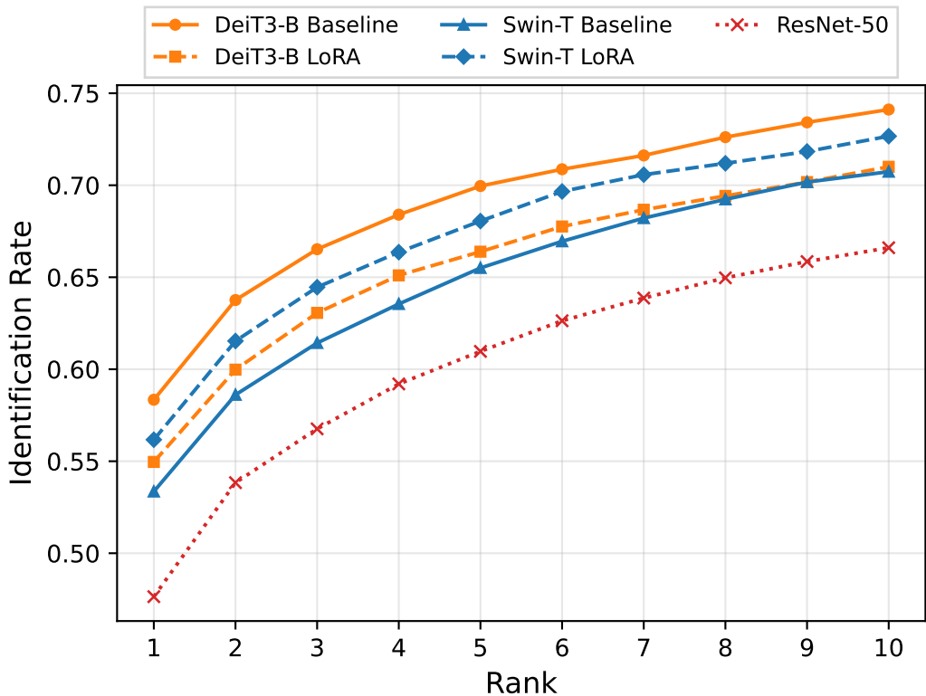
CMC Curves — Top Models on TinyFace
