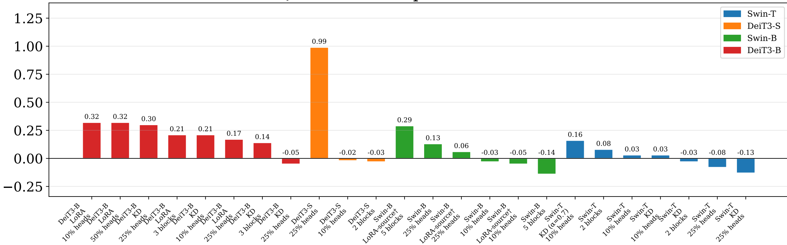
INT8 Quantization Impact on Pruned Models
