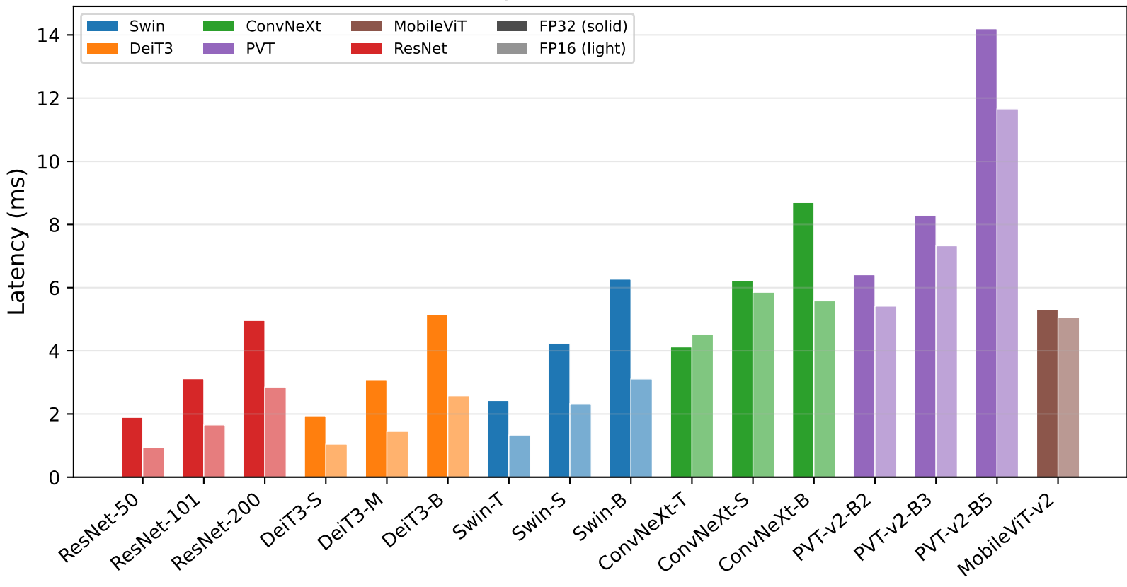
Jetson Orin Nano Latency — FP32 vs FP16 (batch size 1, 96×96)
