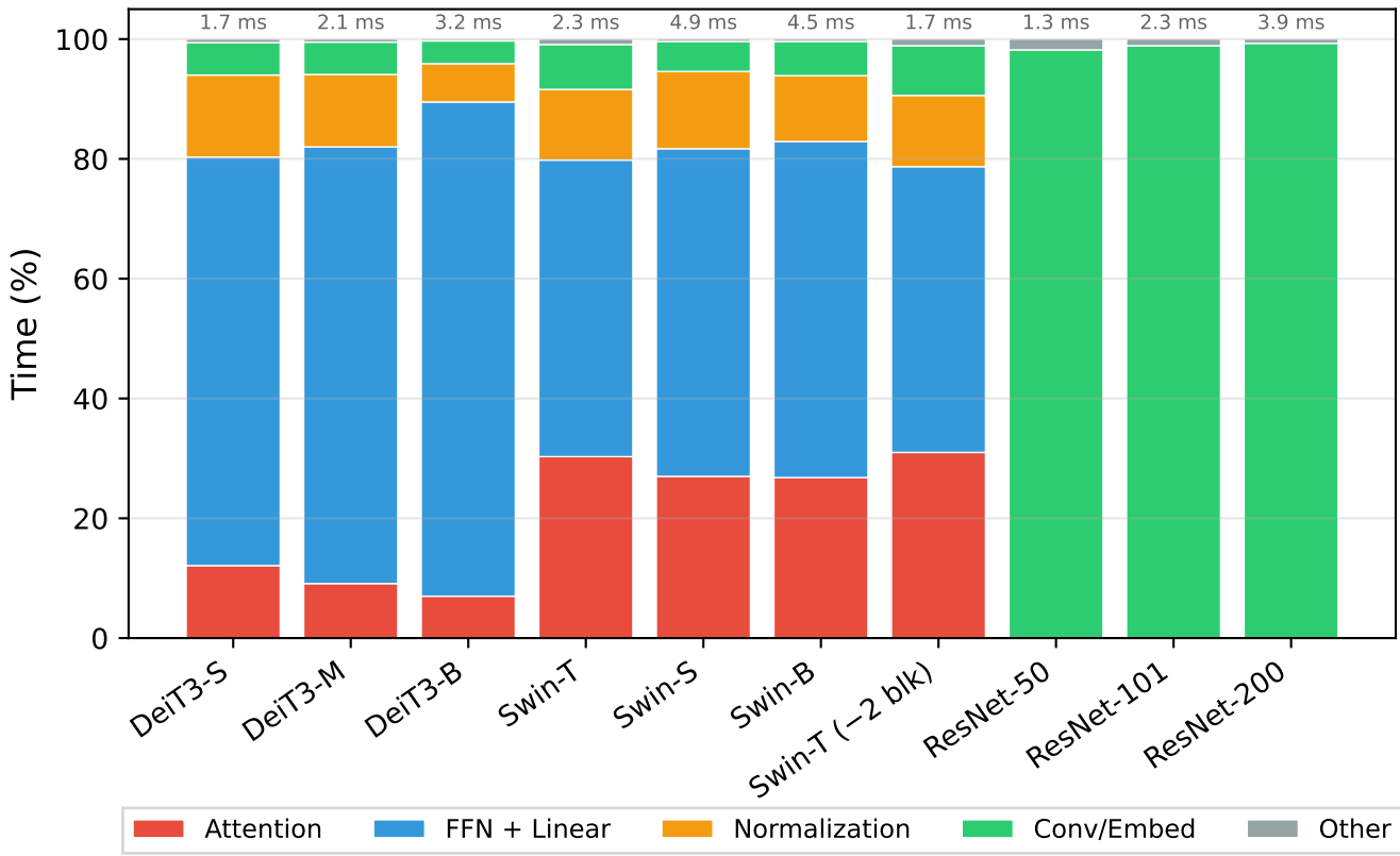
Per-Layer Time Breakdown (FP16, Jetson Orin Nano)
