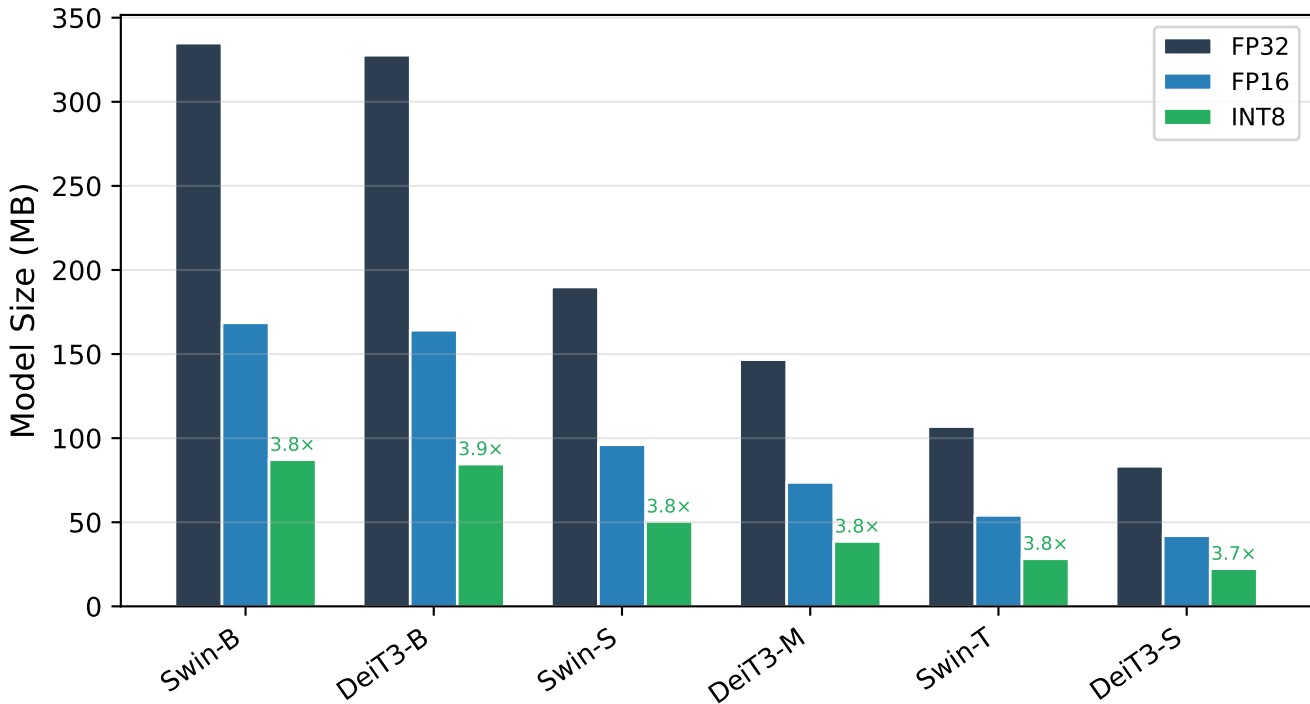
Model Size Reduction: FP32 \rightarrow FP16 \rightarrow INT8
