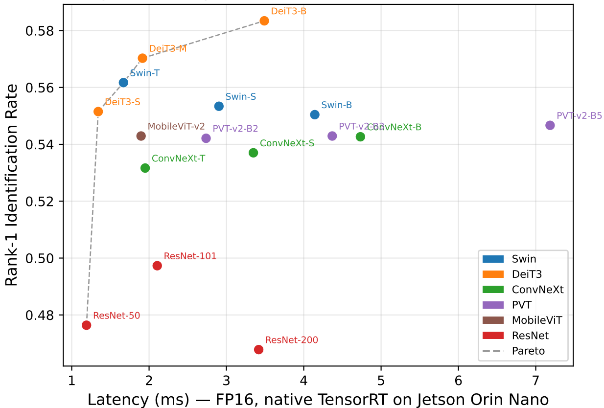
Accuracy vs. Latency — Baseline Models (FP16, unified native TRT)
