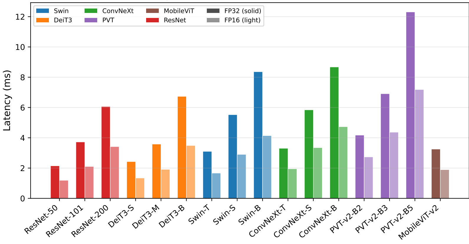
Jetson Orin Nano Latency — native TensorRT, FP32 vs FP16 (batch size 1, 96×96)
