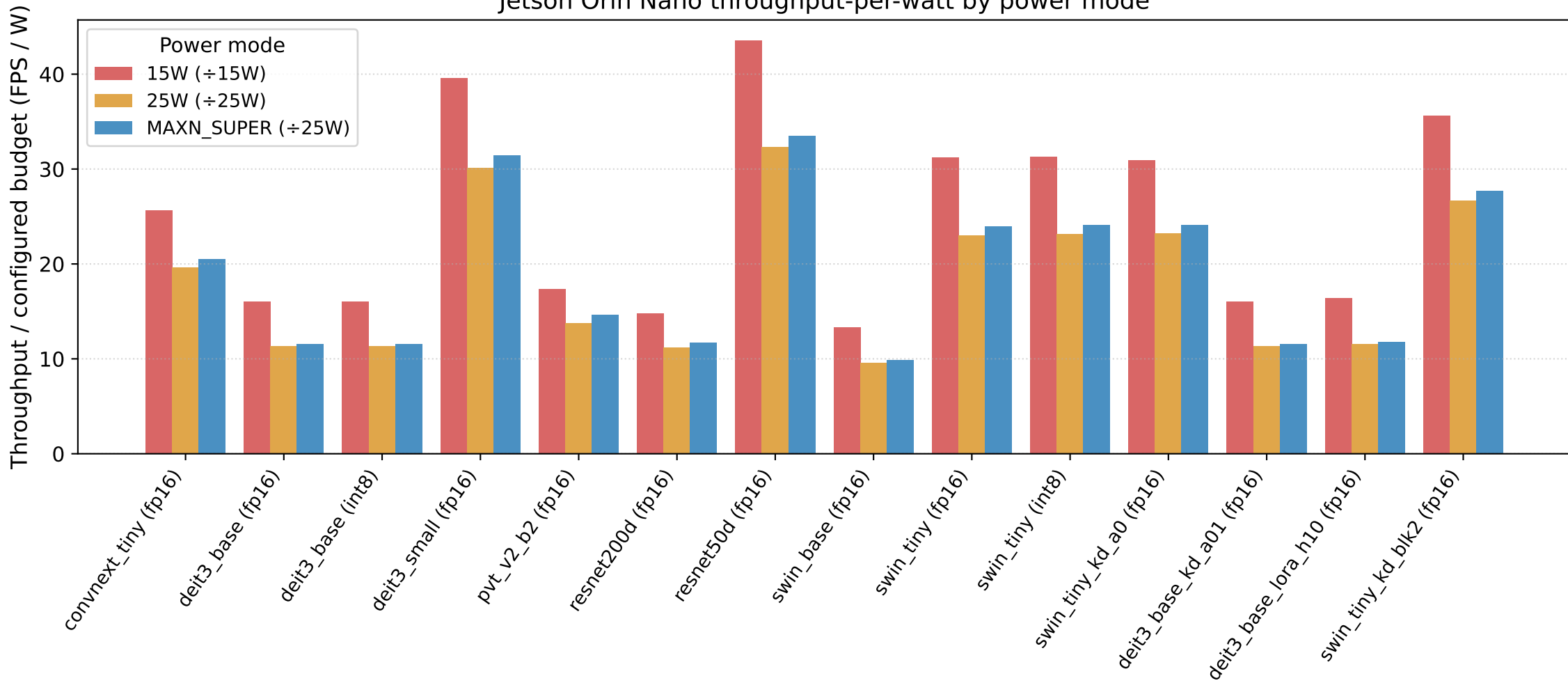
Jetson Orin Nano throughput-per-watt by power mode
