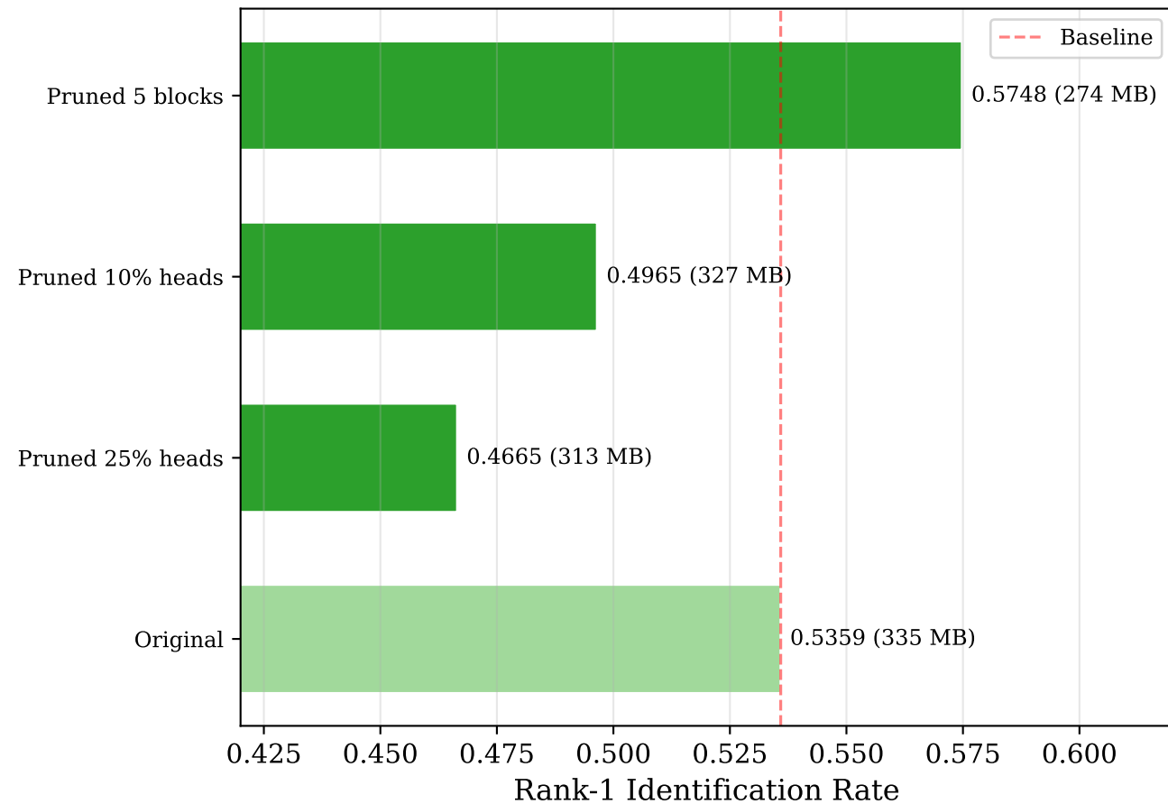
Swin-Base
