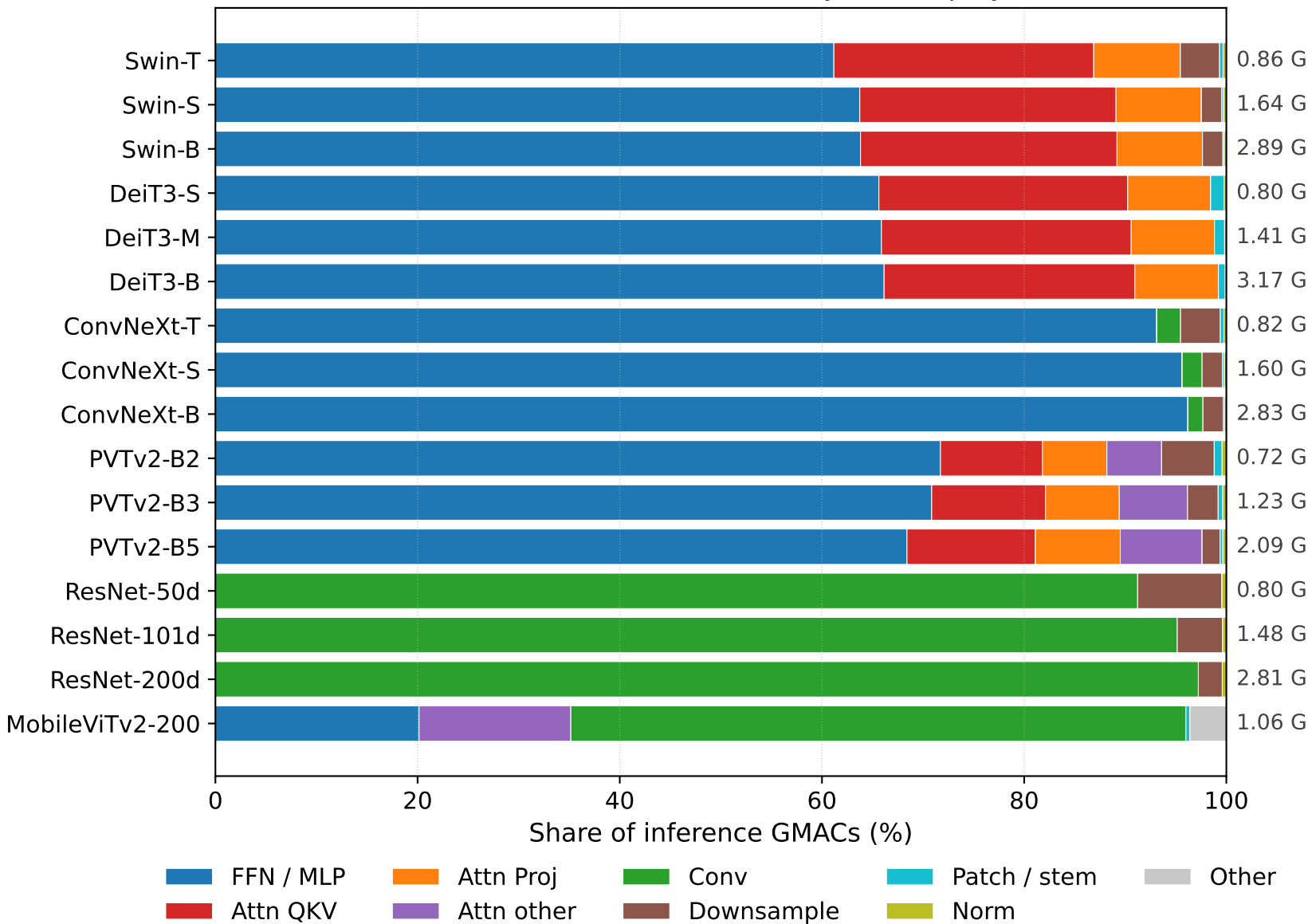
GMACs breakdown at 96 × 96 (TinyFace deployment)
