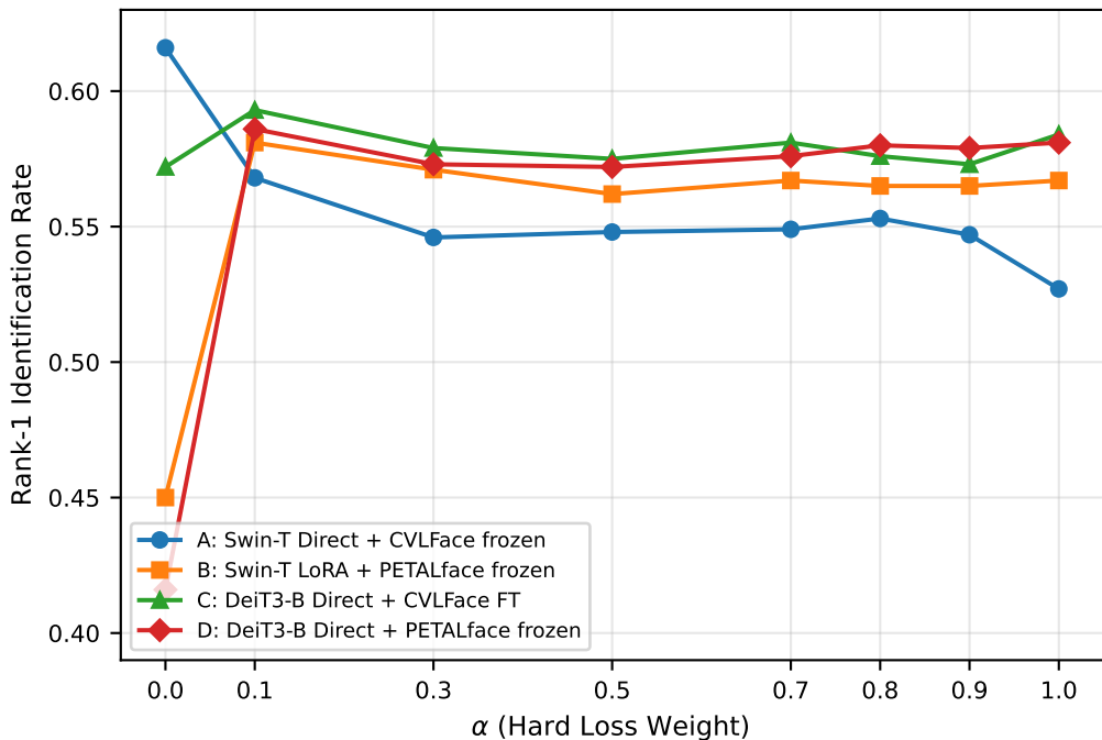
KD Loss Mixing ( \alpha ) Ablation
