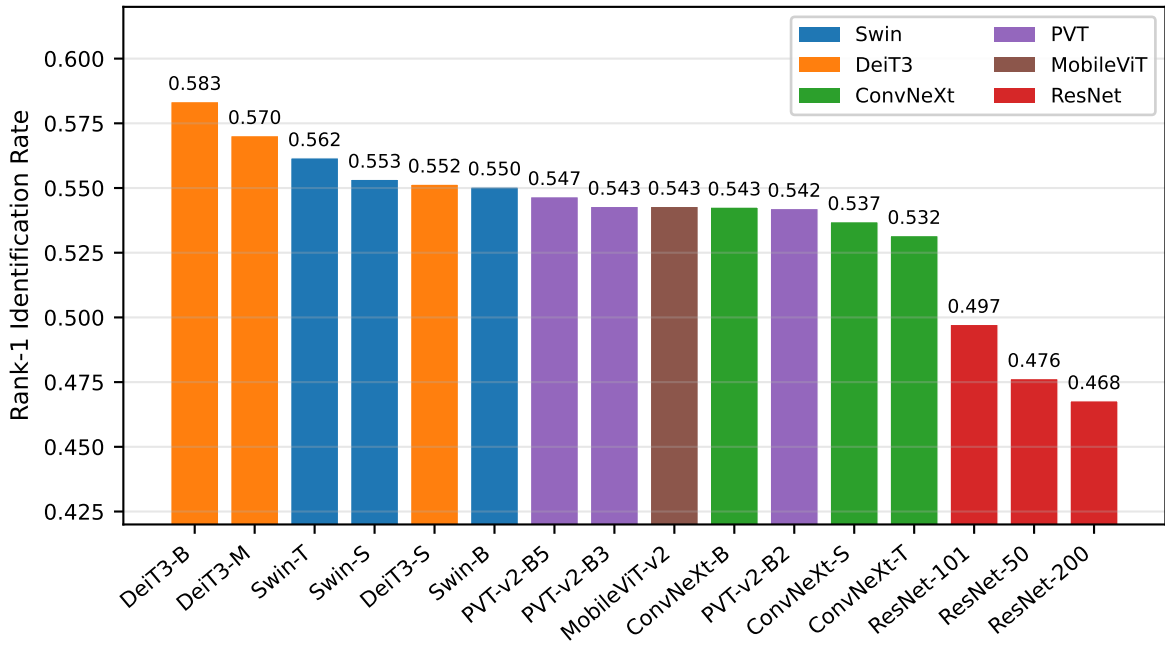
Baseline Model Comparison on TinyFace (96×96)
