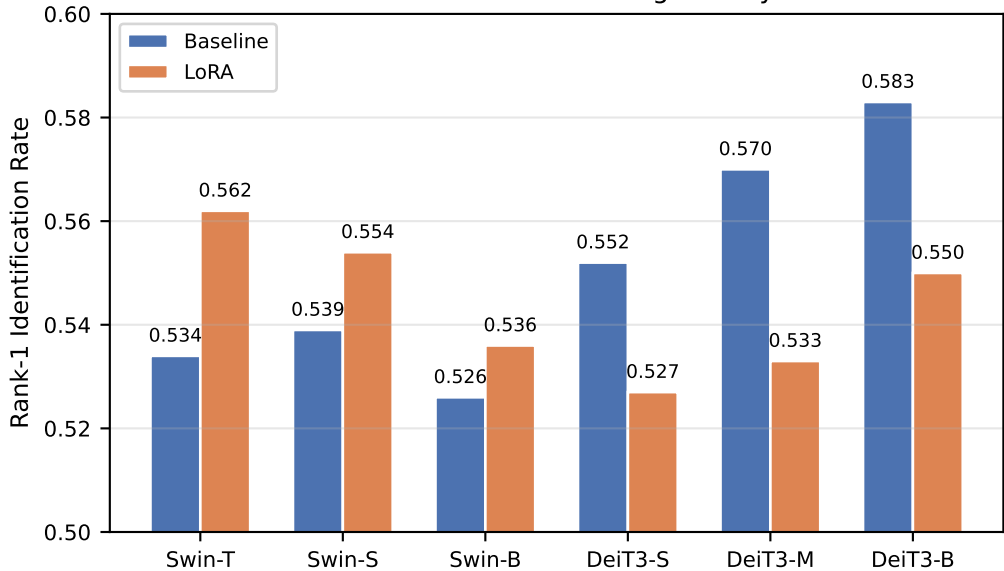
Baseline vs. LoRA Fine-Tuning on TinyFace
