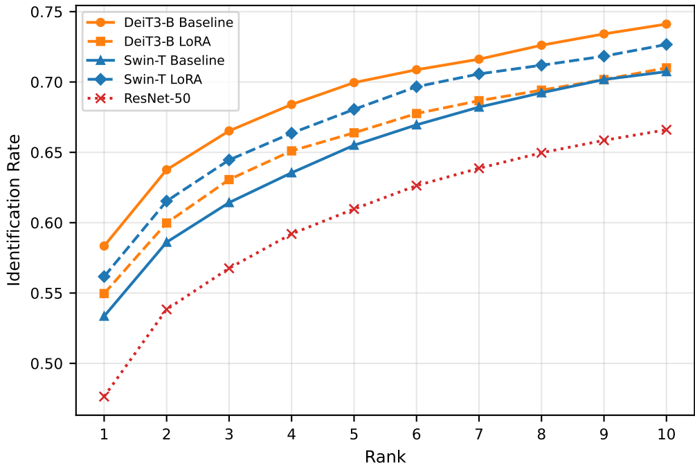
CMC Curves — Top Models on TinyFace
