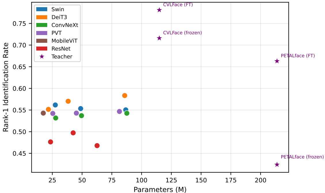
Model Size vs. Accuracy on TinyFace
