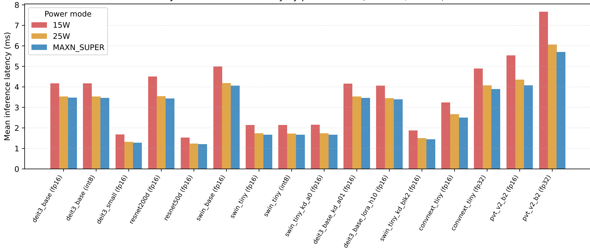
Jetson Orin Nano latency by power mode (batch=1, 96×96)
