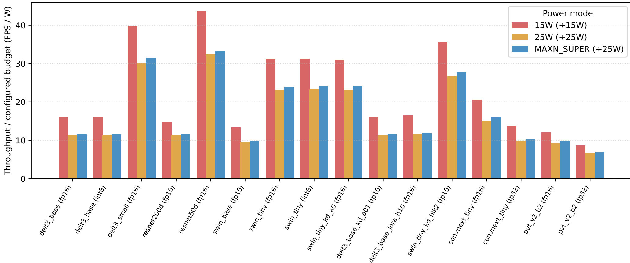
Jetson Orin Nano throughput-per-watt by power mode
