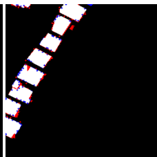
CDMaskFormer
