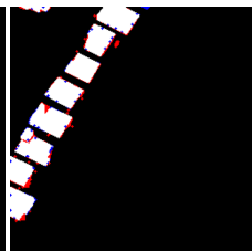
SCACD-Mamba
