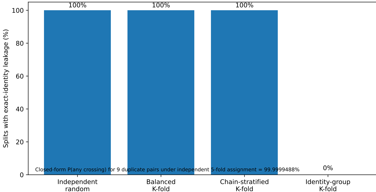
Exact-identity leakage across split strategies (1,000 simulations each)
