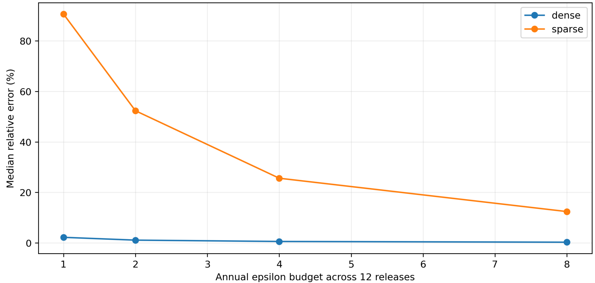
User-level DP utility and release-budget trade-off
