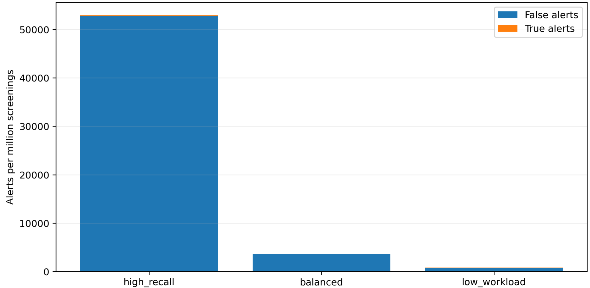
Operational alert workload at 0.01% prevalence
